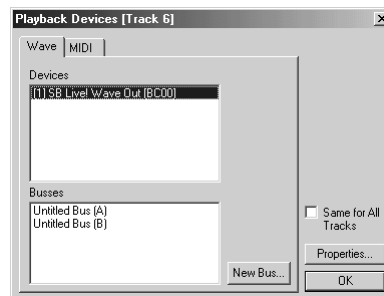
The Wave Tab of the Playback Devices Dialog
