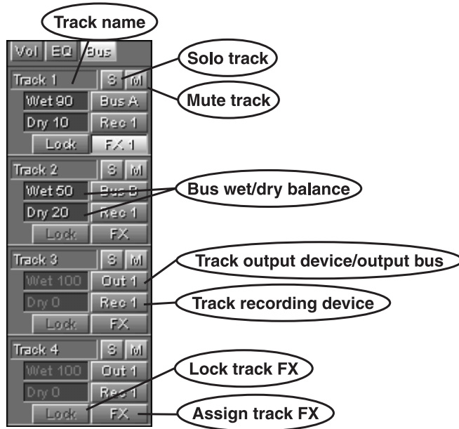
Track Controls set to the Bus Tab
