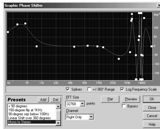
Graphic Phase Shifter Dialog
