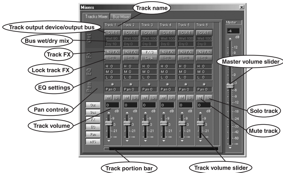
Tracks Mixer Window
