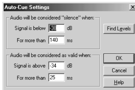
Auto-Cue Settings Dialog
