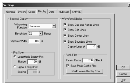
The Display Tab of the Settings Dialog
