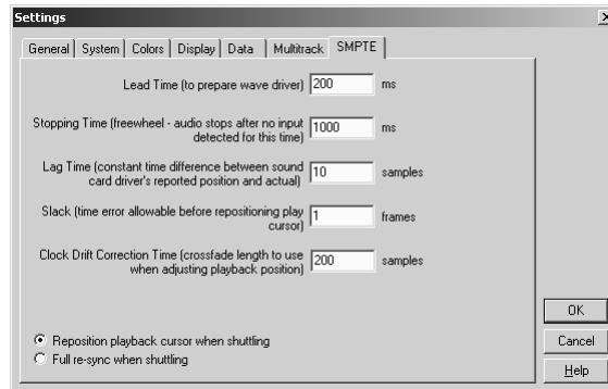
The SMPT E Tab of the Settings Dialog
