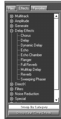
The Effects Pane of the Organizer Window with "Group By Category" active
