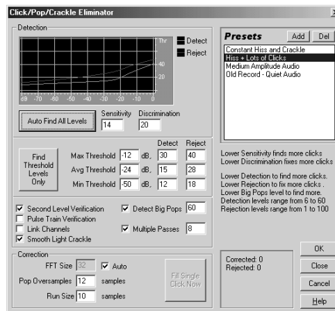
Click/Pop Eliminator Dialog
