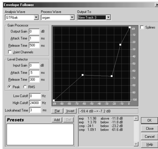
Envelope Follower Dialog
