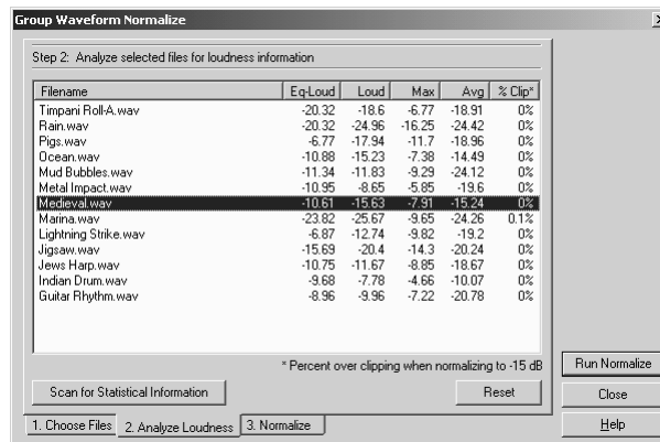
The Analyze Loudness Tab of the Group Waveform Normalization Dialog
