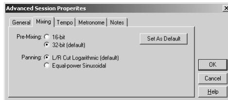
The Mixing Tab of the Advanced Session Properties Window
