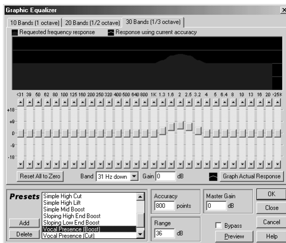
Graphic Equalizer Dialog (30 Bands Tab)
