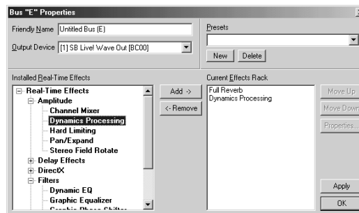
Bus Properties Dialog
