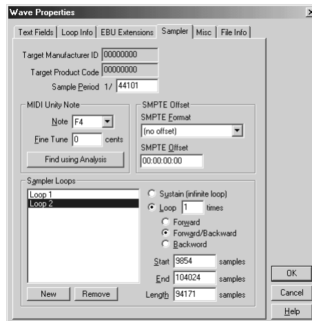
Wave Properties Dialog - Sampler Tab
