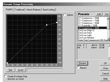
Dynamics Processing Dialog - Graphic Tab
