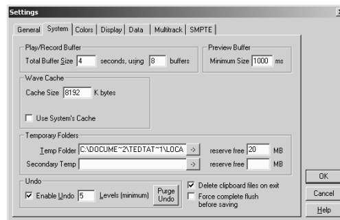
The System Tab of the Settings Dialog
