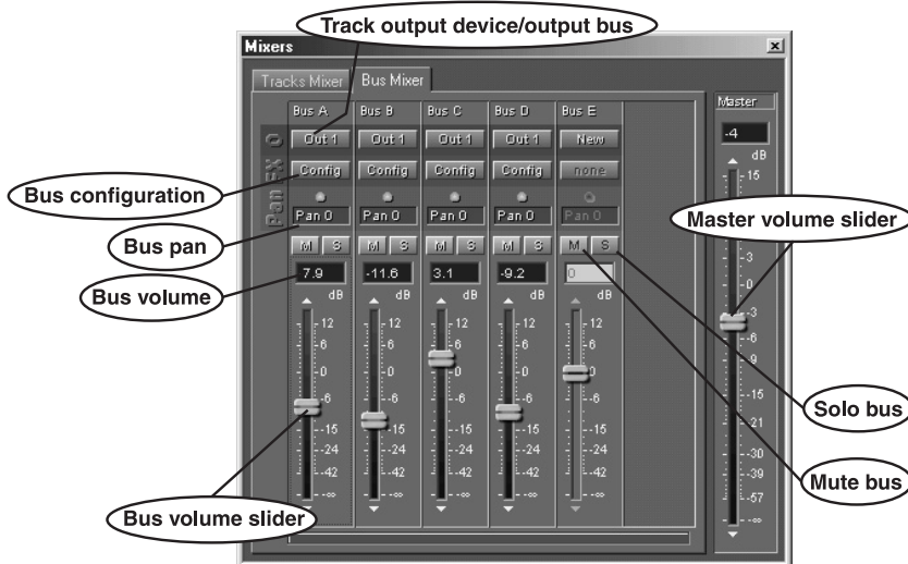
Bus Mixer Window
