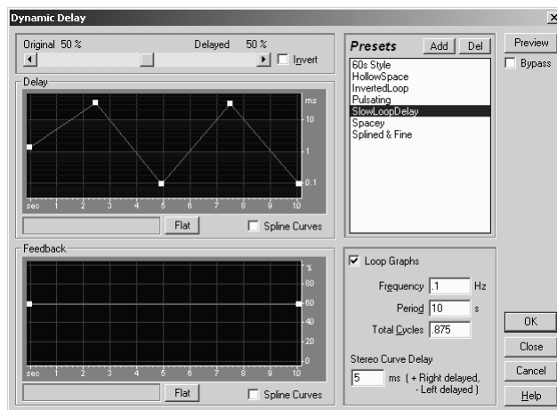
Dynamic Delay Dialog
