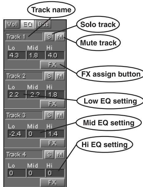
Track Controls set to the EQ Tab
